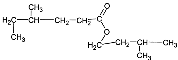
3-methyl-butyl-4-methylhexanoate
