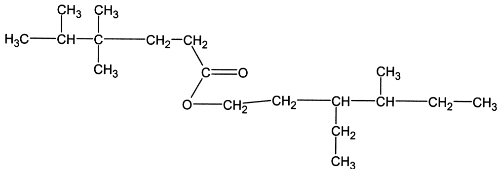
3-ethyl-4-methyl-hexyl-4,4,5-trimethylhexanoate
